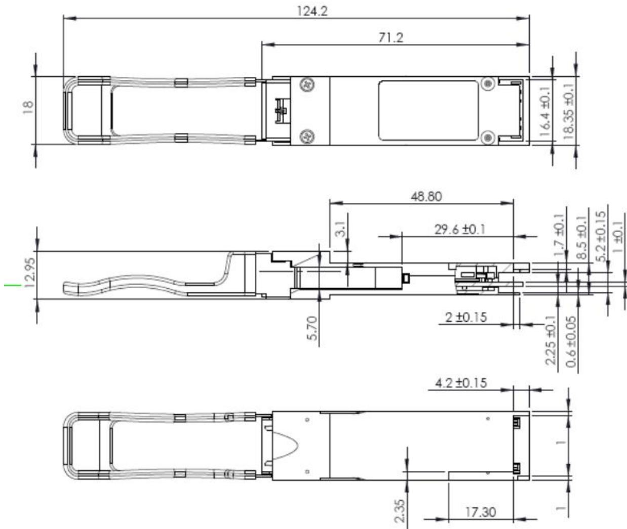
Figure 5: Mechanical Dimensions
